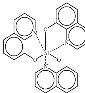
\text{Alq}_3
