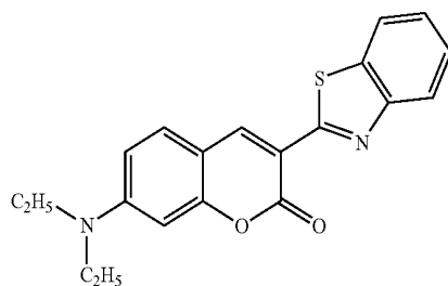
Coumarin6
