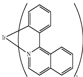
\text{Ir}(\text{piq})_3
